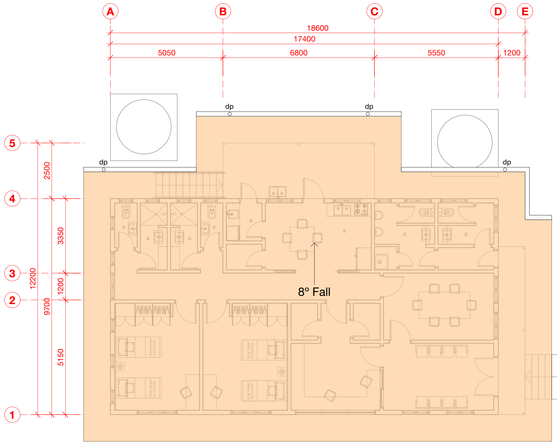
Total Roof Area: 275m 2
