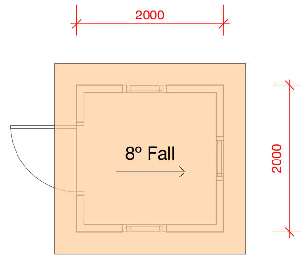
Total Roof Area: 7m 2
