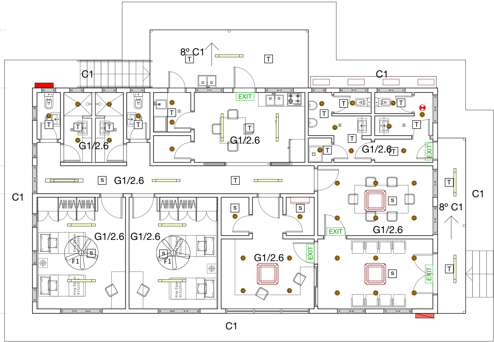
1 PROPOSED REFLECTED CEILING PLAN SCALE: 1:100
