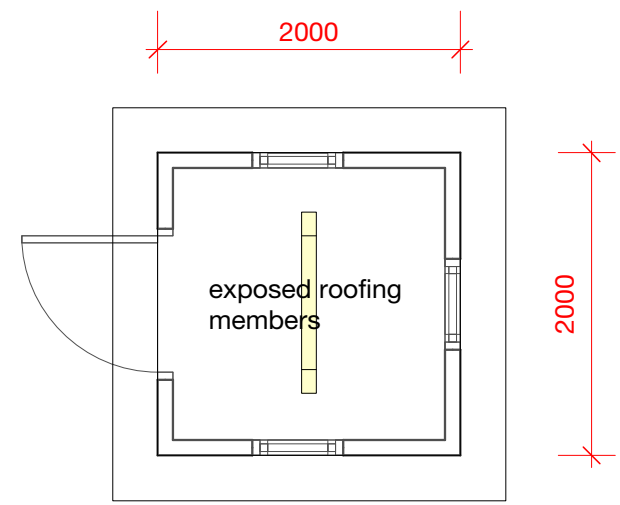
3 TYPICAL SECURITY BOOTH REFLECTED CEILING PLAN SCALE: 1:50
