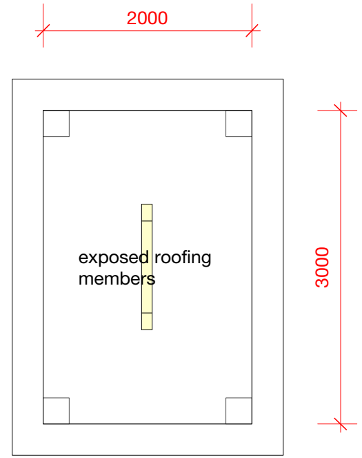
2 PROPOSED WAITING BURE REFLECTED CEILING PLAN SCALE: 1:50
