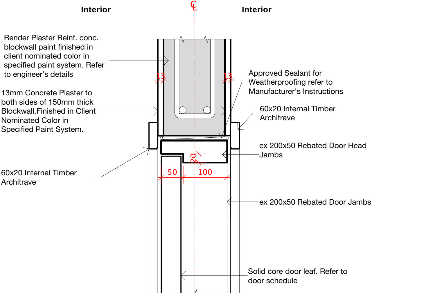
1 INTERNAL SINGLE SWING DOOR HEAD DETAIL SCALE: 1:5
