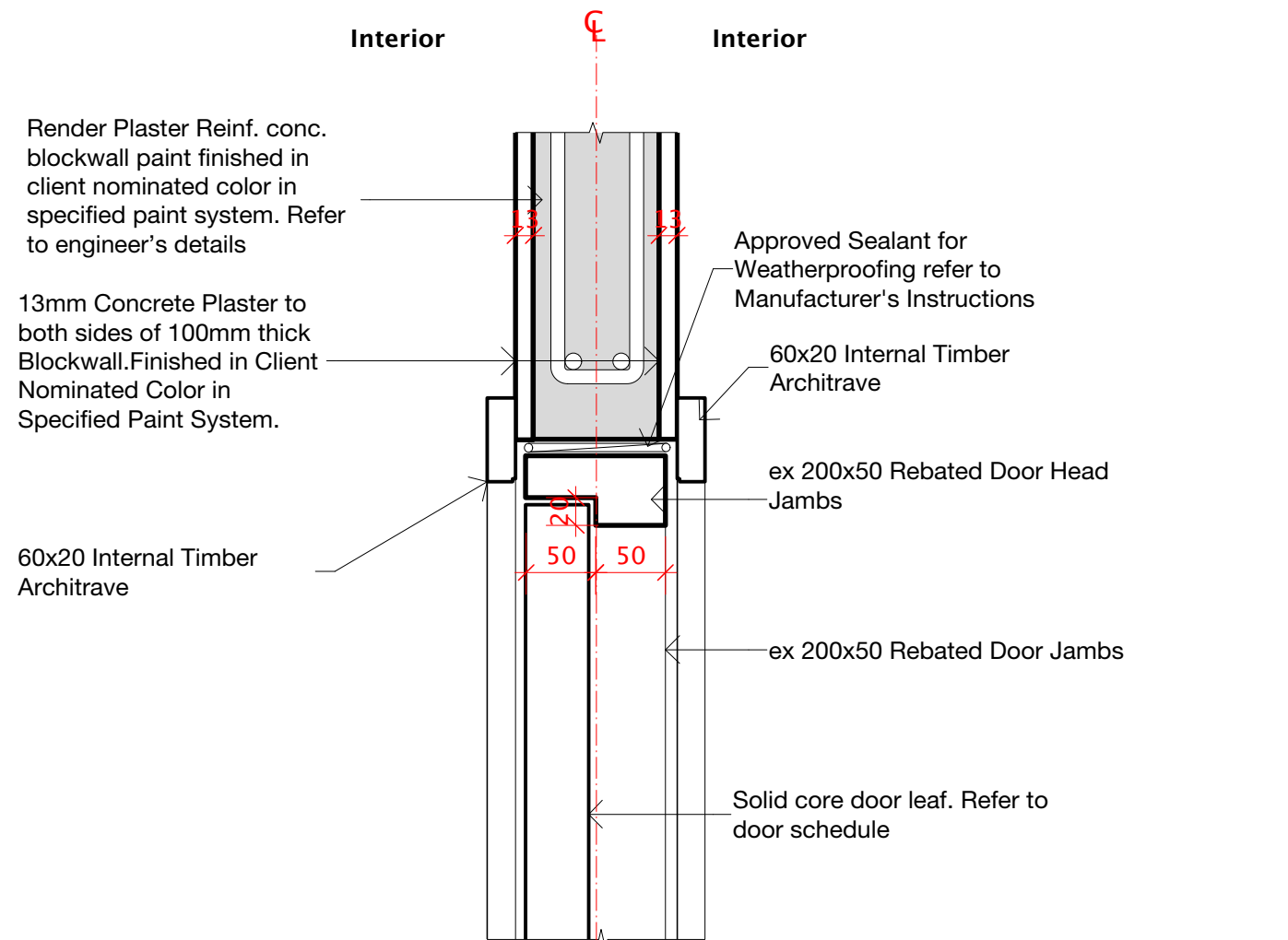
1 INTERNAL SINGLE SWING DOOR HEAD DETAIL SCALE: 1:5
