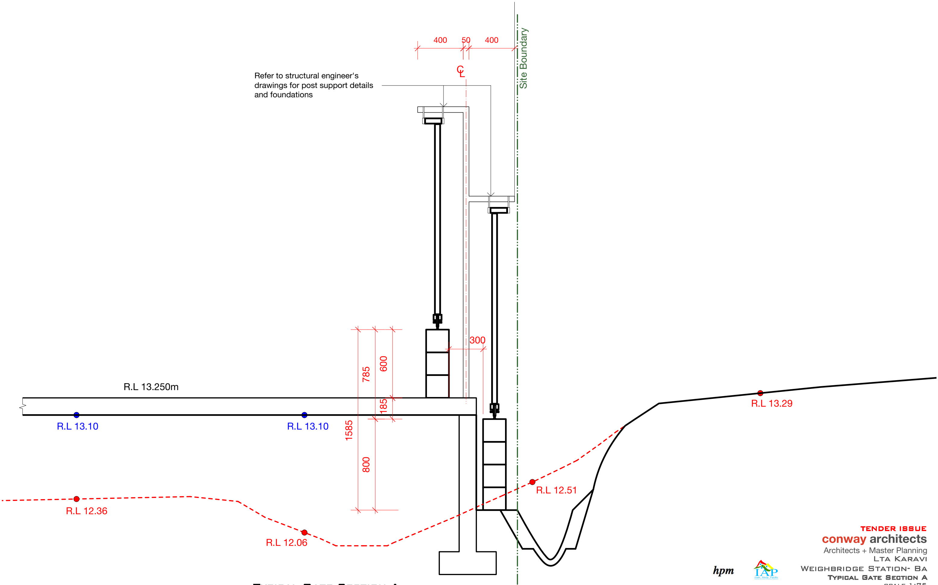
TYPICAL GATE SECTION A
